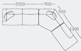
Angled modular with open end (LH // RH) – overall size: 4200 × 900/ 2300mm
