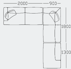
L shaped Modular 5 seater (LH // RH) – overall size: 2900 × 900/ 3100mm
